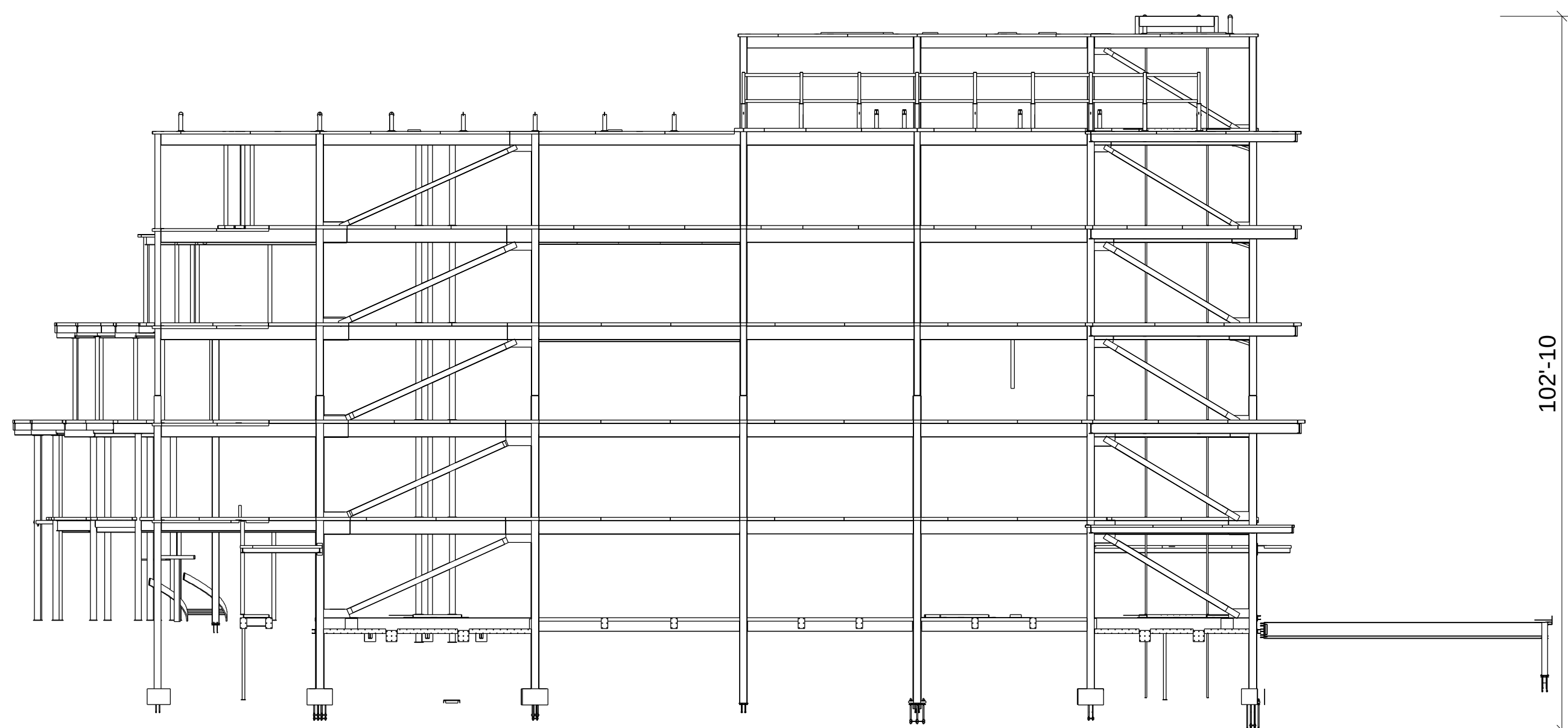
ELEVATION VIEW (ALONG GRID P8)
