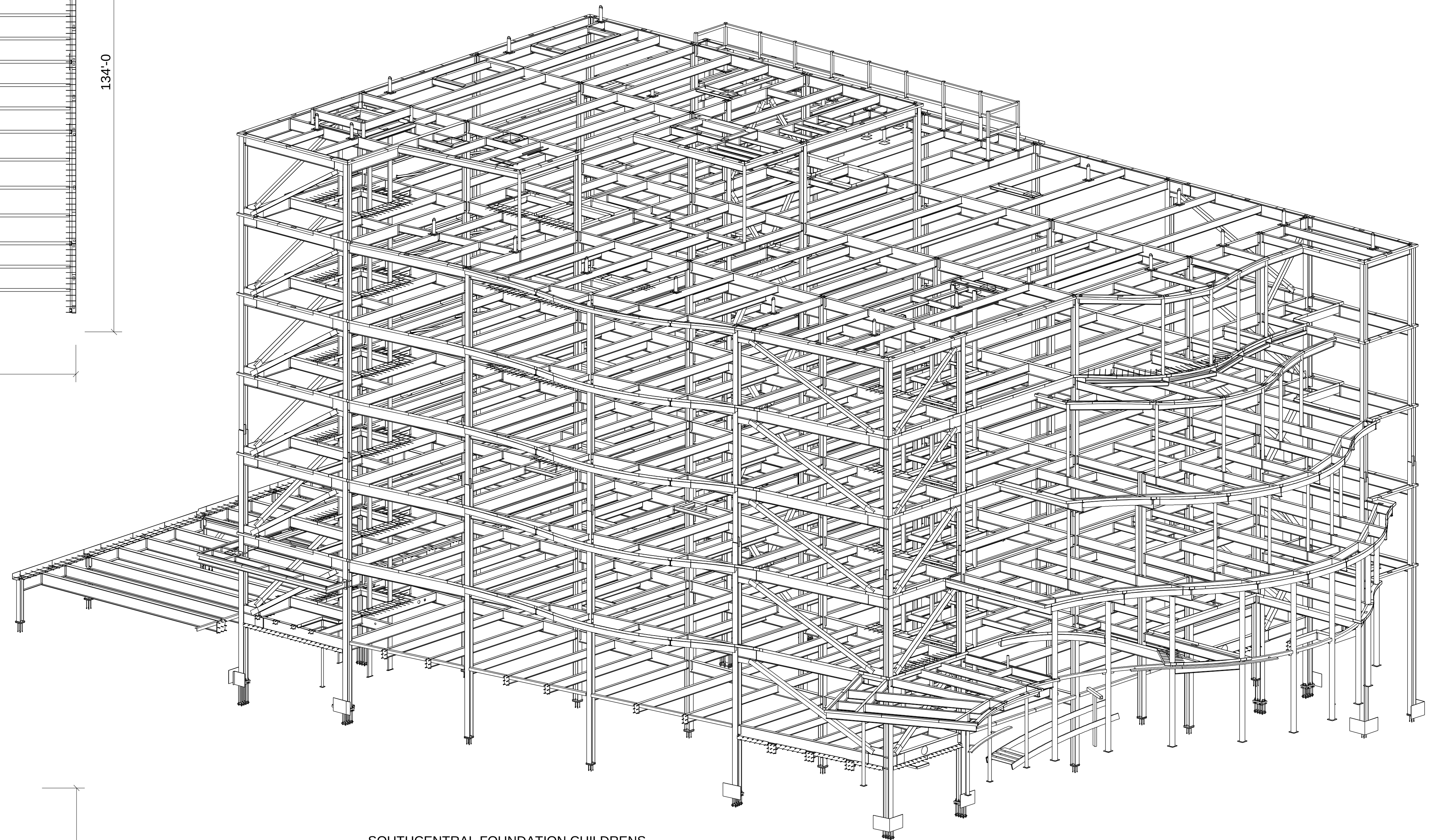
SOUTHCENTRAL FOUNDATION CHILDRENS DENTAL CLINIC BUILDING - PERSPECTIVE VIEW (WEIGHT APROX. 720 TONS)
