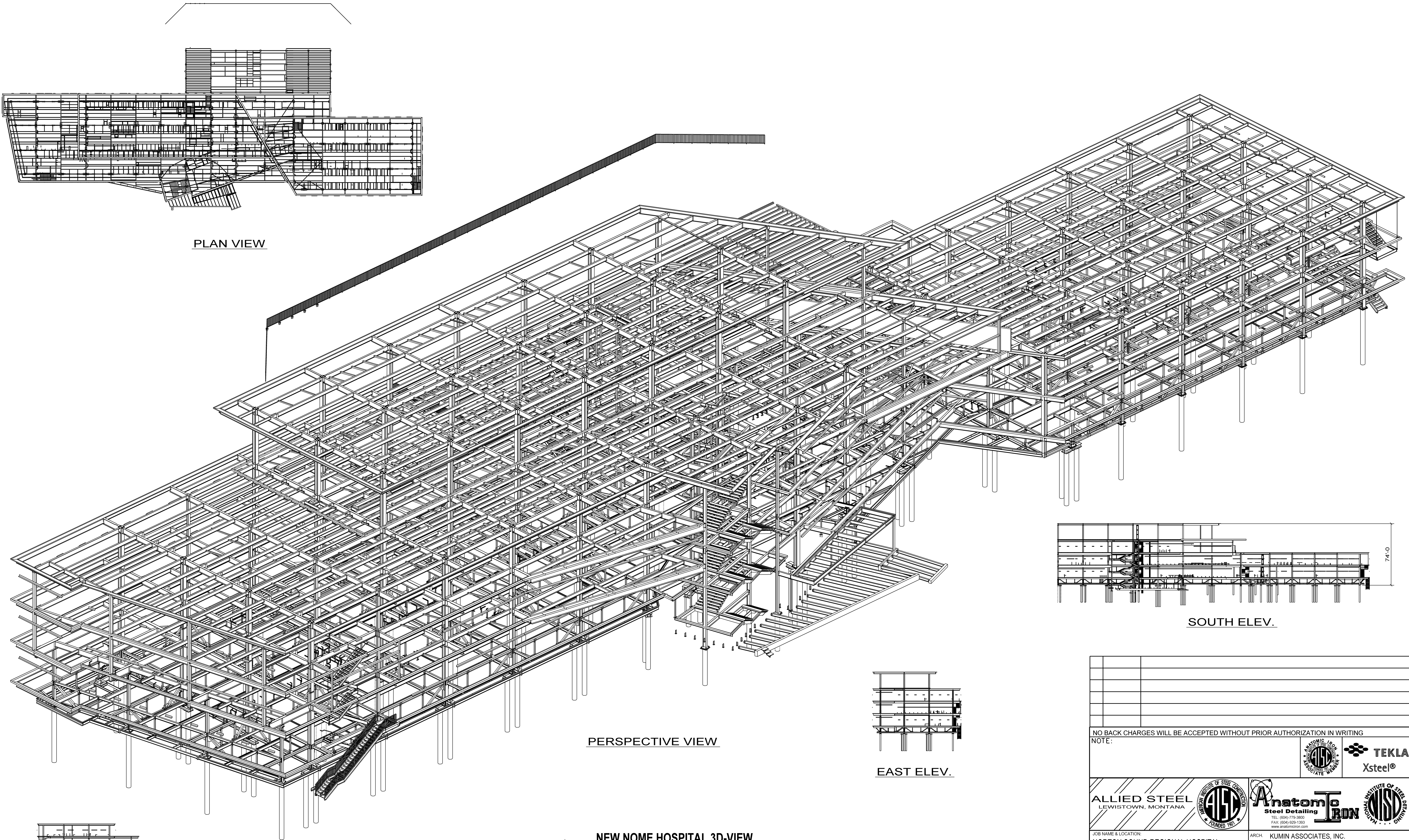
NEW NOME HOSPITAL 3D-VIEW NORTON SOUND REGIONAL HOSPITAL 3D VIEW (APPROX. WT- 1386 TONNES)
